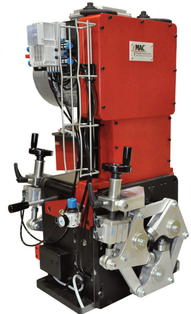
Rotary Probe Tester, shown above, can be used with MultiMac SM electronics to test for long, seam type defects in tube, bar or rod in continuous operations, or straight and cut.
