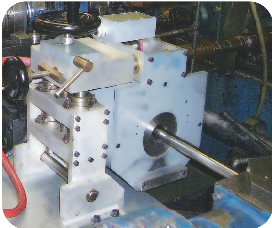
352 Coil Platform with Encircling Coil testing welded tube for short defects
