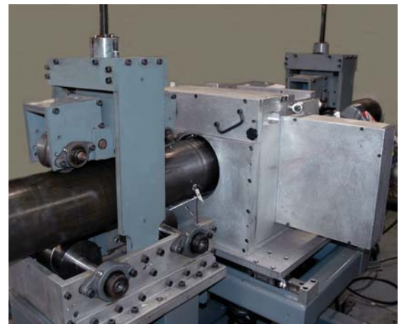
Shown above is the Model 750 Rotomac ® rotary test head for inspecting 7-1/2" (190.5 mm) diameter cut lengths, often in-line with straighteners or installed in a separate test station. Installations can be completely automatic, including marking and sorting devices. The rotary is usually mounted in conjunction with MAC Slide/Elevating and Drive Mechanisms to position the rotary housing and move the material accurately through the test head.
