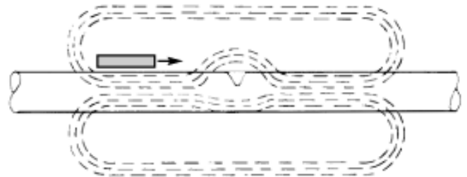
FIGURE 6 LONGITUDINAL MAGNETIZATION
