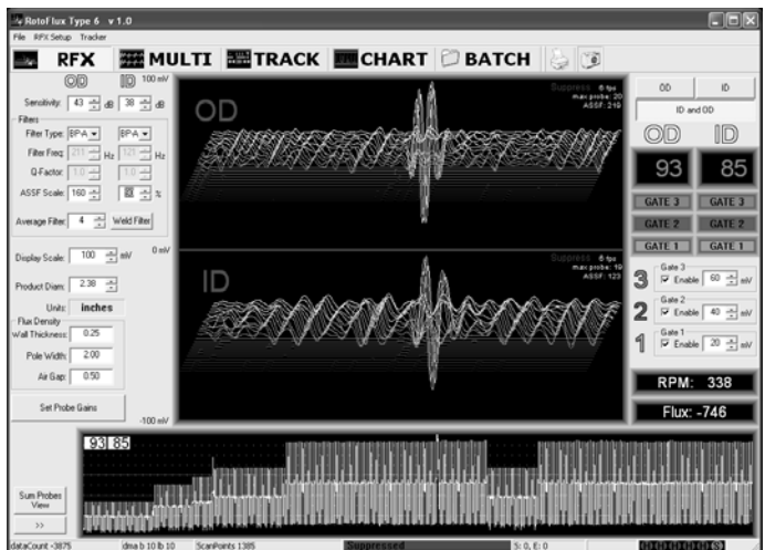
Picture 3 Signal from a 10% OD notch on a 2 3/8" diameter tube
