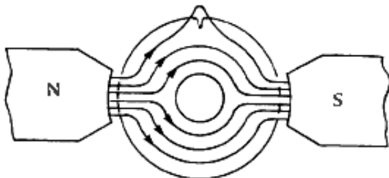
FIGURE 1 Outside diameter crack causes flux lines to "leak" beyond the tube.
