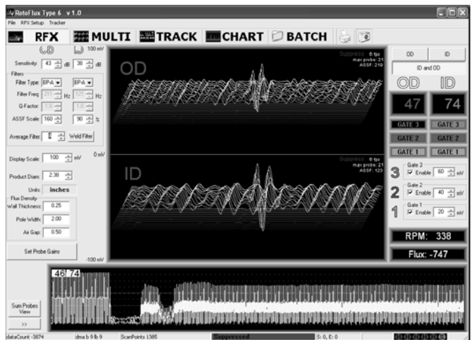
Picture 2 Signal from a 10% ID notch on a 2 3/8" diameter tube
