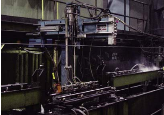
Squirter type ultrasonic inspection station on a weld-line at Wheatland Tube, Arkansas. MAC Echomac electronics are operating with this test system.
